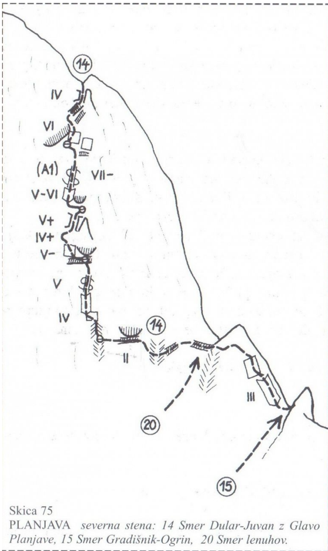
Planjava, severna stena: 14 Smer Dular-Juvan z Glavo Planjave, 15 Smer Gradišnik-Ogrin, 20 Smer
